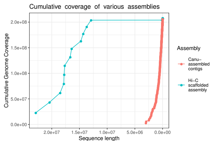
Figure 4 Cumulative coverage of initial and final (scaffolded) C. columbae genome assemblies, illustrating the improvement in contiguity by scaffolding with Hi-C data. All scaffolds in the assembly are plotted largest to smallest, from left to right. The x-axis indicates cumulative length of an assembly, and the y-axis corresponds to the cumulative portion of the genome covered by initial contigs (red dots) and final scaffolds (blue dots).
